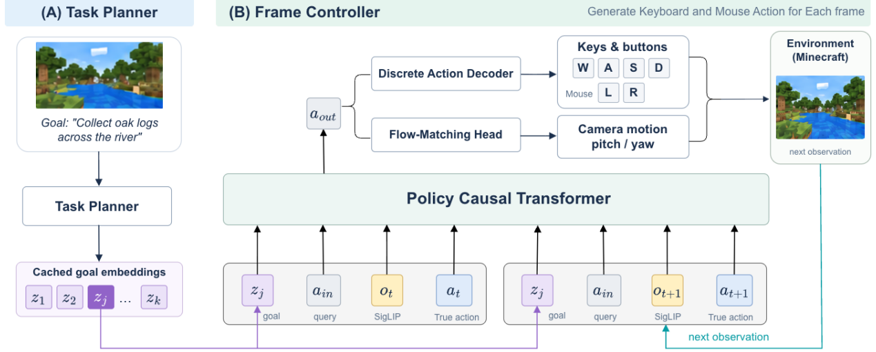
Figure 2 Overview of TaskFrame , a hierarchical planner–controller agent that separates task-level planning from frame-level control. (A) Task Planner. A vision–language model decomposes a high-level goal (e.g., “collect oak logs across the river”) into an ordered sequence of atomic goals, each terminated by a special goal token. The hidden states at these tokens are cached as goal embeddings z_1, \dots, z_k . (B) Frame Controller. A per-frame autoregressive policy. Each frame consumes the active goal embedding z_j , an action-query token a_{in} , a SigLIP image token o_t , and the action a_t , which only later frames attend to. A causal Transformer aggregates them into the action-output token a_{out} , which is decoded into discrete keyboard and mouse-button presses and continuous camera motion. The planner runs once per high-level goal, while the controller acts at every game step.
