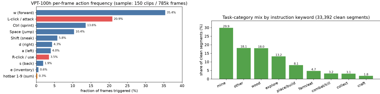
Figure 4 Statistics of the controller training data. Left: per-frame action frequency on a sample of 150 clips (785K frames). Right: task category mix of clean segments, grouped by instruction keyword.
