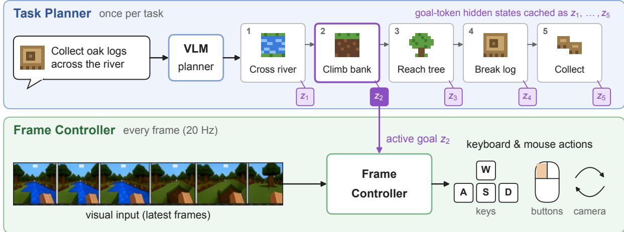
Figure 1 Overview of TaskFrame. Once per task, the task planner decomposes a high-level instruction into ordered atomic goals, each terminated by a special goal token whose hidden state is cached as a goal embedding. At every frame, the frame controller takes the embedding of the active goal and the latest visual input and emits native keyboard-and-mouse actions.
