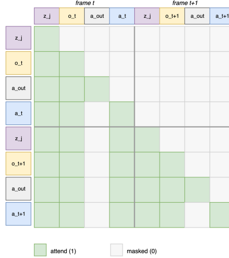
Figure 5 Causal attention mask of the frame controller, adopted from Yue et al. (2026) and shown for two consecutive frames. Rows are query tokens and columns are key tokens; green cells are attended and gray cells are masked. Each frame contributes the goal condition z_j , the visual token o_t , the action-output token a^{\text{out}} , and the ground-truth action a_t . No token attends to a^{\text{out}} , and a^{\text{out}} at frame t attends to previous ground-truth actions but not to the same-frame action a_t .
